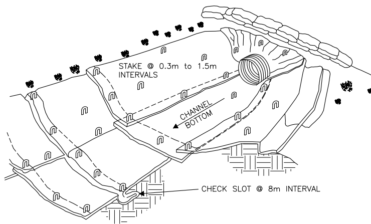
ISOMETRIC VIEW
