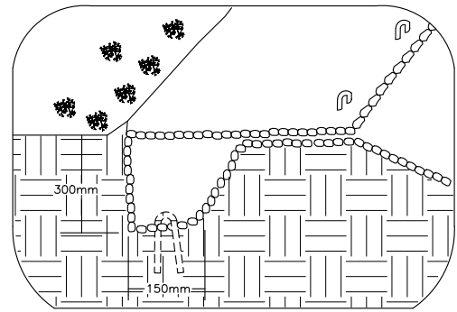
TERMINAL SLOPE AND CHANNEL ANCHOR TRENCH
