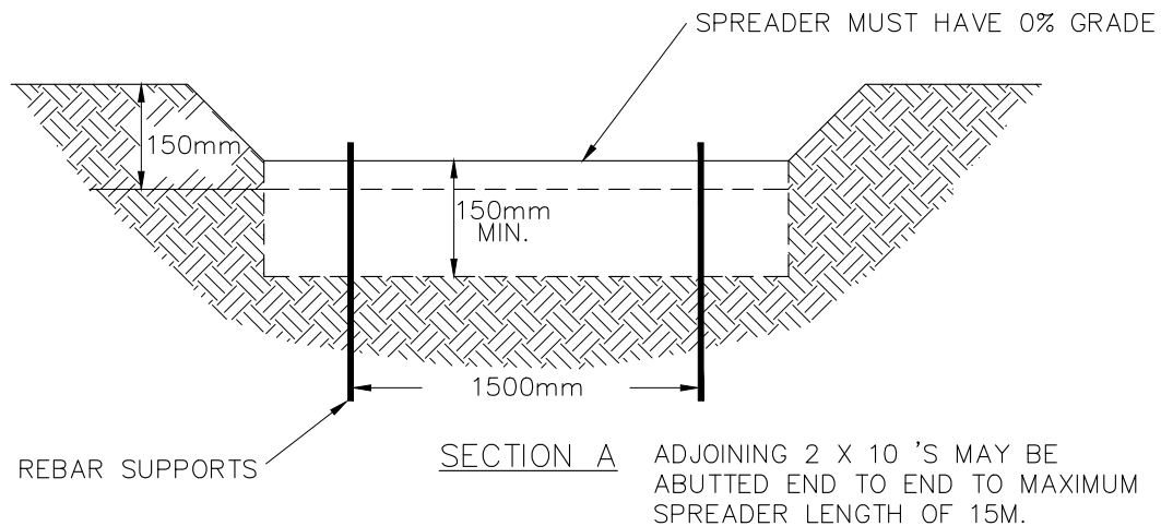
CROSS SECTION
