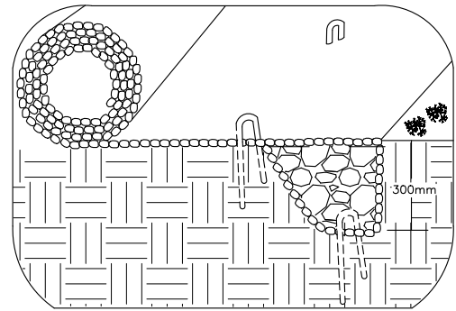
INITIAL CHANNEL ANCHOR TRENCH
