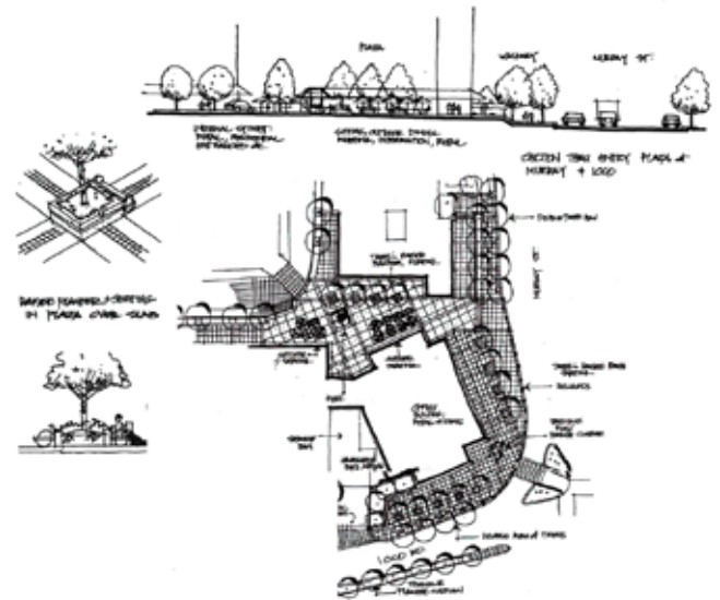
Figure 9: Conceptual Plan of Intersection, loco Road & Murray St.
